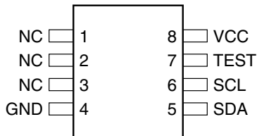
8-lead SOIC
